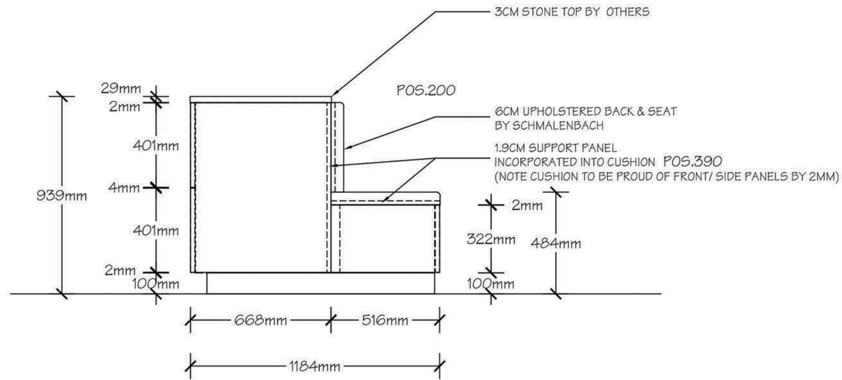
SIDE ELEVATION
