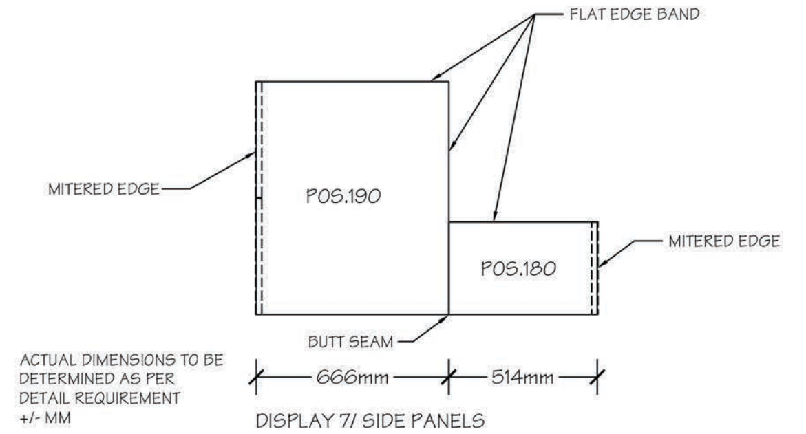
SIDE PANEL(S) ELEVATION
