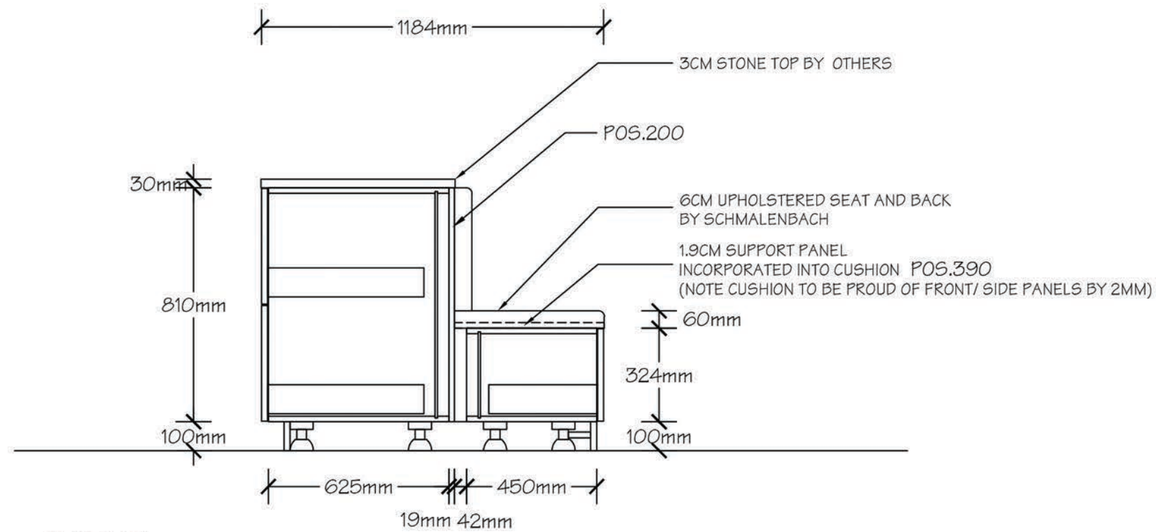
SECTION -
