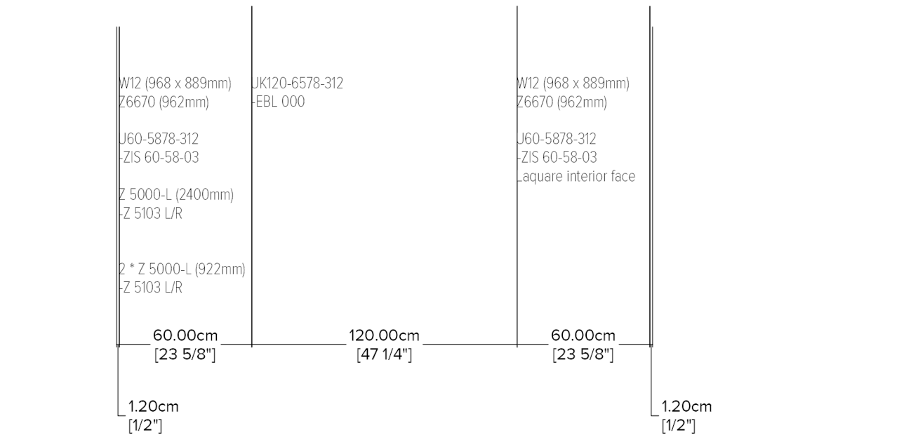
D ELEVATION
