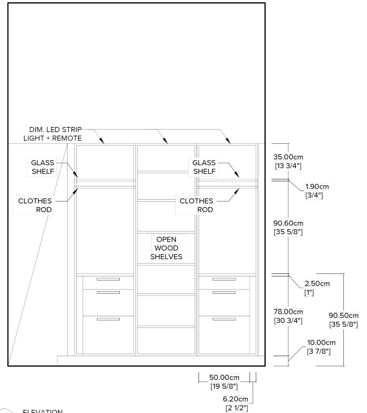
B ELEVATION ART CABINETS CLOSED
