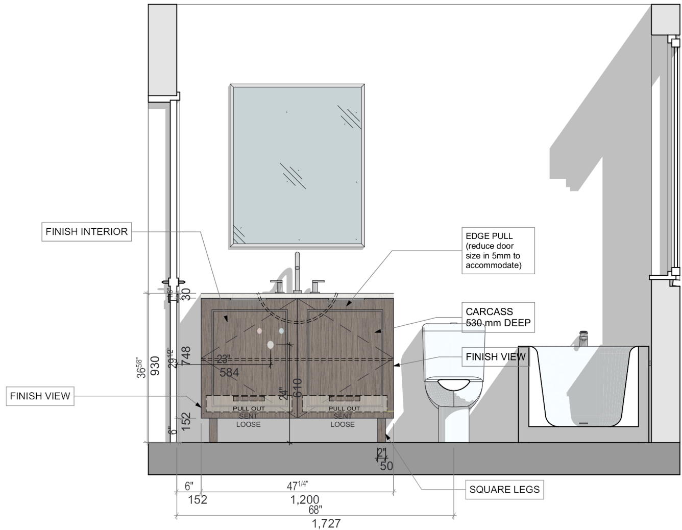
BH-8 Elevation
