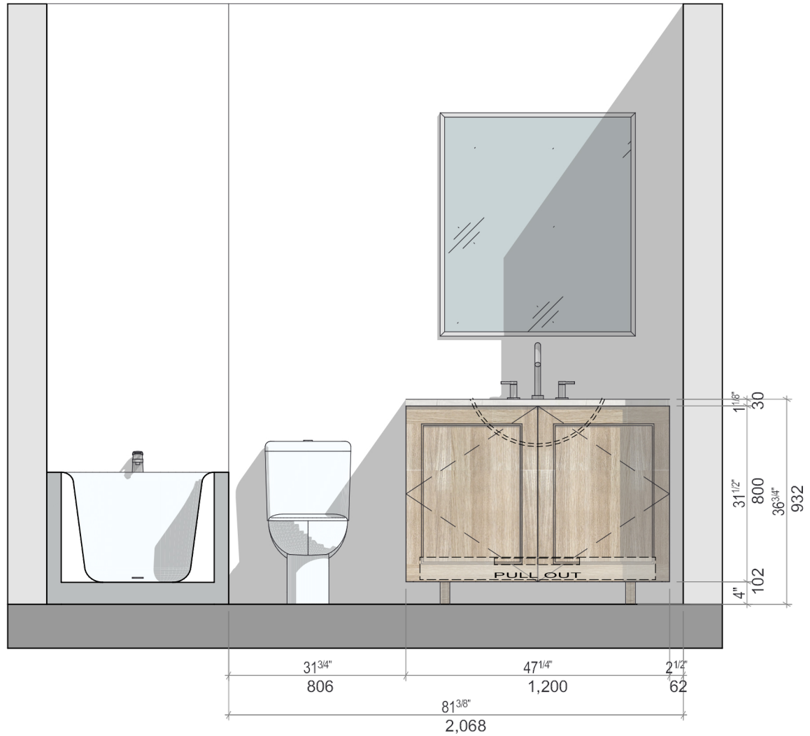
BH-013 Elevation
