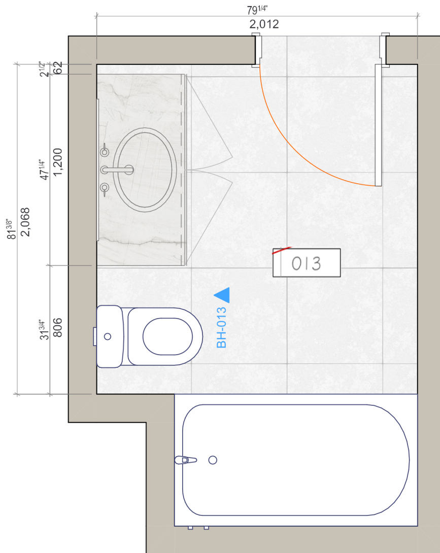
0. FLOOR PLAN
