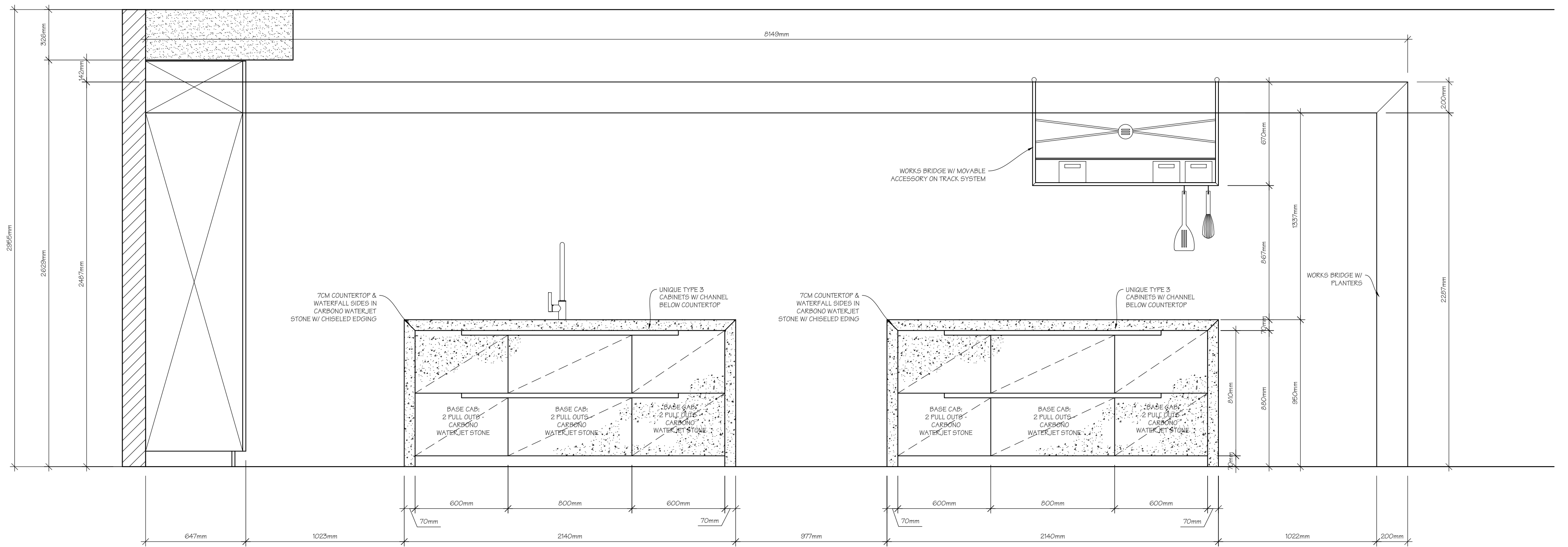
HOUSTON SHOWROOM - DISPLAY #7 ELEVATION D
