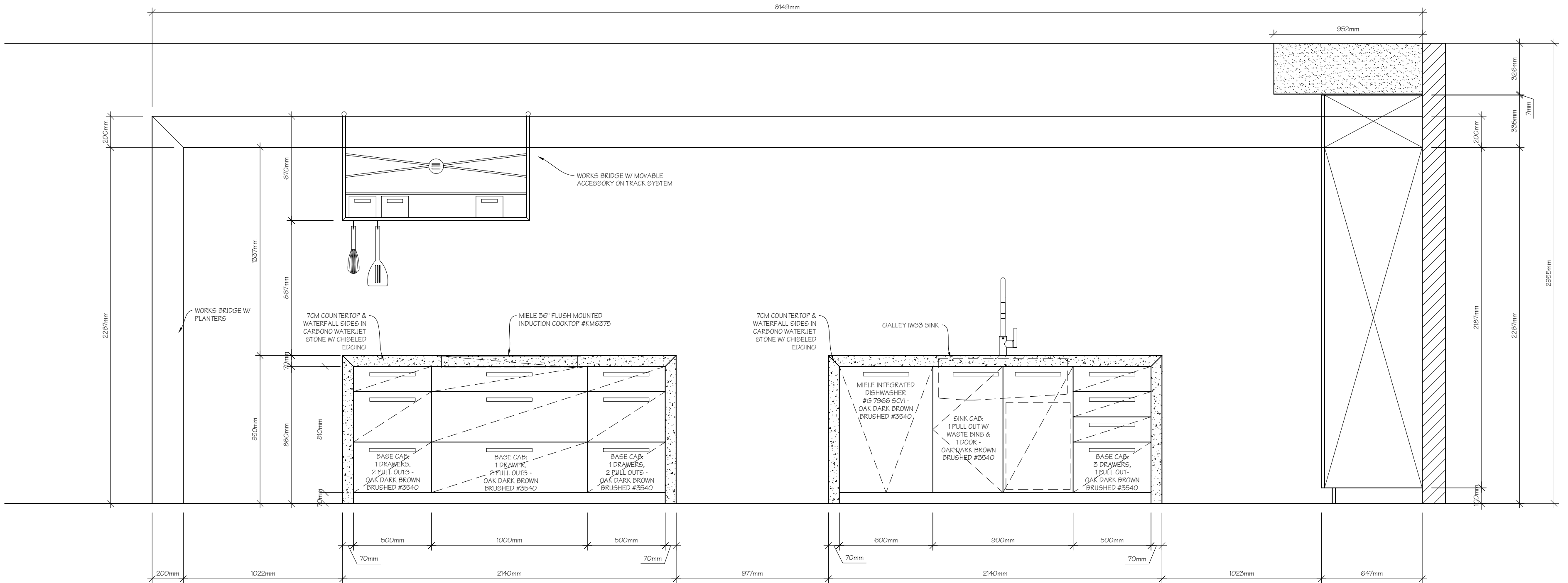
HOUSTON SHOWROOM - DISPLAY #7 ELEVATION C
